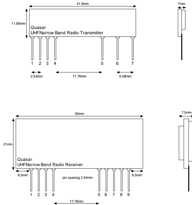
Figure 6: FM Narrow Band Transmitter and Receiver
